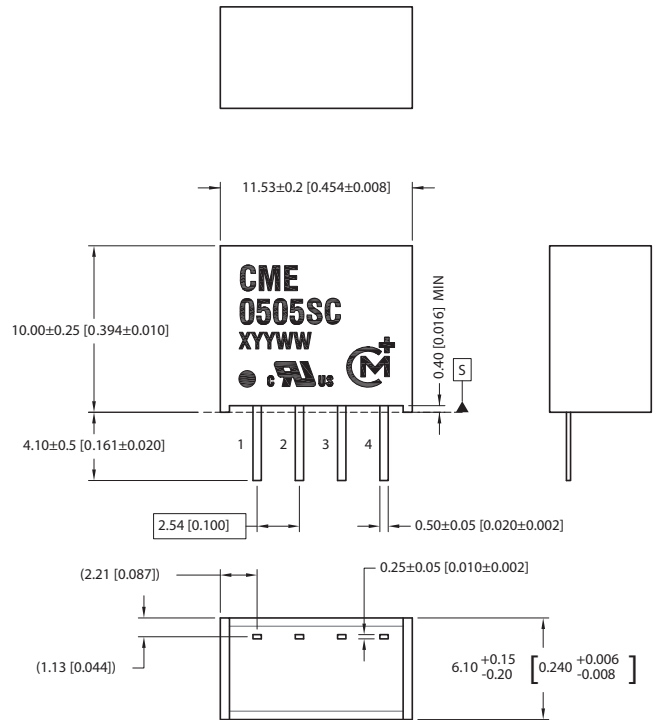
SC Package
