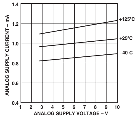
TPC 24. CMP402 Analog Supply Current vs. Analog Supply Voltage
