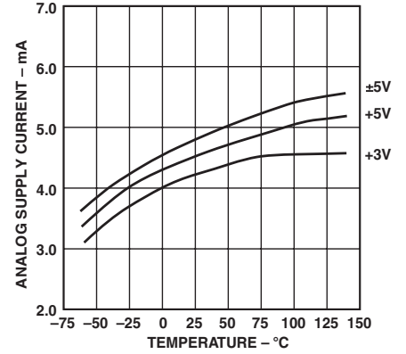
TPC 21. CMP401 Analog Supply Current vs. Temperature
