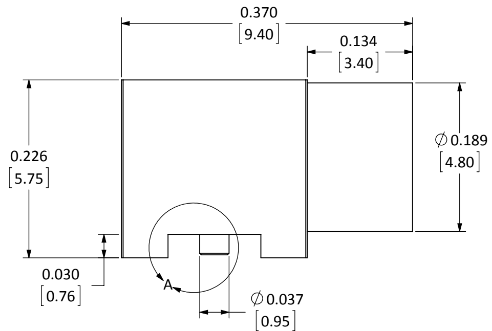
SIDE VIEW
