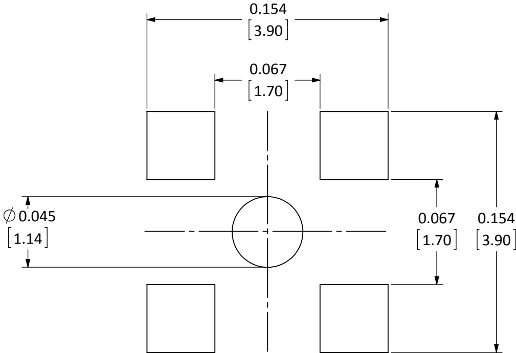
RECOMMENDED FOOTPRINT
