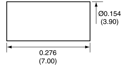
CRIMP RING
