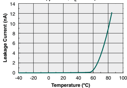
Typical Leakage vs. Temperature ( I_F=0\text{mA} , V_L=250\text{V} )
