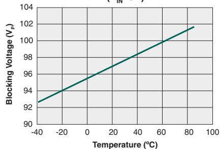
Typical Blocking Voltage vs. Temperature ( V_{IN} = 5V )
