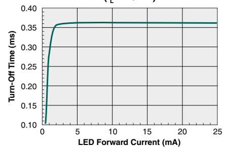
Typical Turn-Off Time vs. LED Forward Current ( I_L=120\text{mA} )
