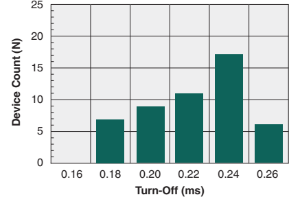
Typical Turn-Off Time (N=50, I_F=20\text{mA} , I_L=1A_{DC} )
