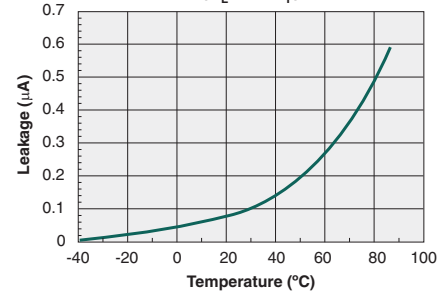
Typical Leakage vs. Temperature Measured Across Pins 1&2 ( V_L=100V_p )
