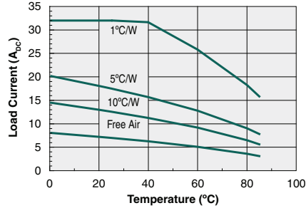
Maximum Load Current vs. Temperature with Heatsink
