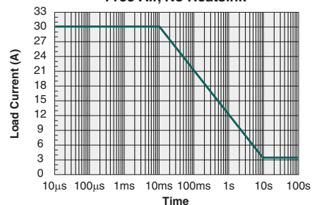
Energy Rating Curve Free Air, No Heatsink
