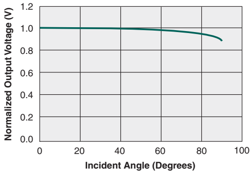
Normalized Open Circuit Output Voltage vs. Incident Angle of Light to Photodiode Surface
