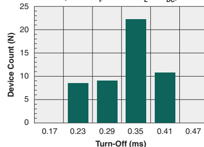
Typical Turn-Off Time (N=50, I_F=20\text{mA} , I_L=1\text{A}_{DC} )
