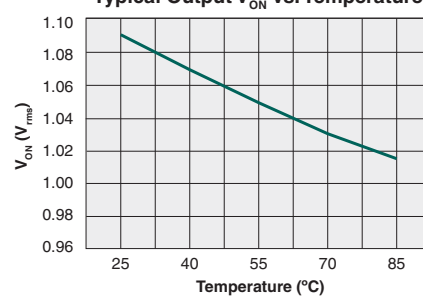
Typical Output V_{\text{ON}} vs. Temperature
