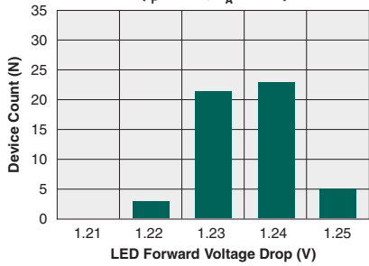
Typical LED Forward Voltage Drop ( I_F=5mA, T_A=25^\circ C )
