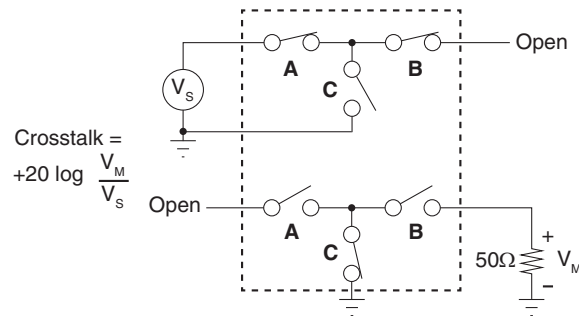
Figure 5. Switch to Switch Cross Talk
