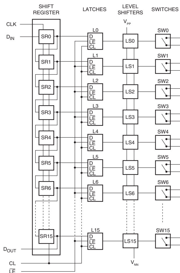
Figure 1. Block Diagram
