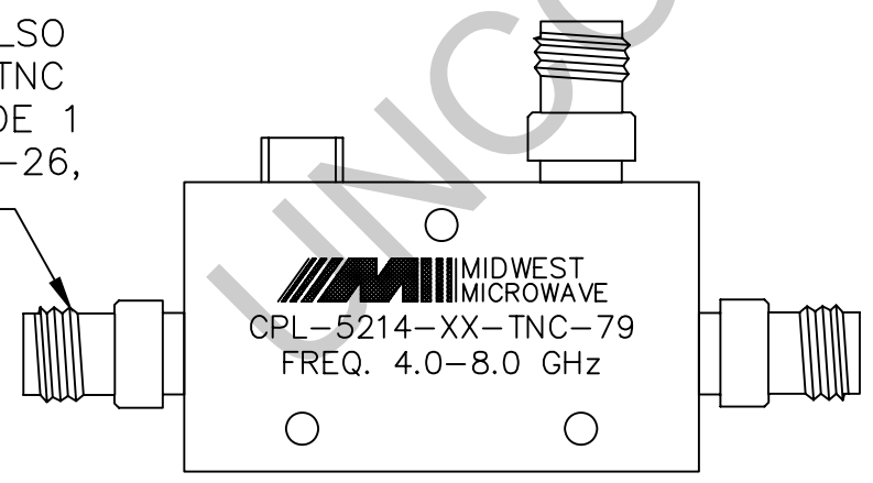
BACKSIDE MARKING
