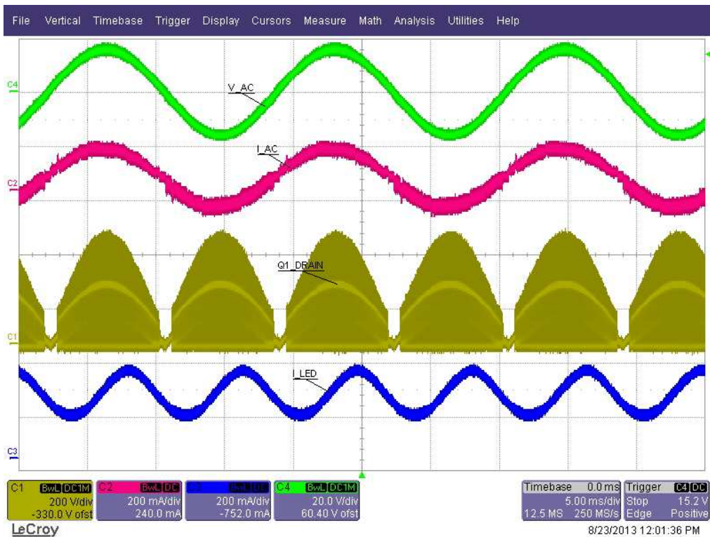
Figure 17. No-dimmer Mode, Steady-state, 120VAC
