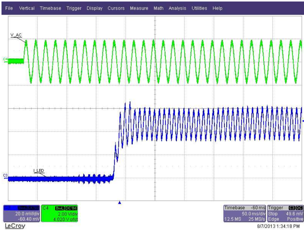
Figure 16. No-dimmer Mode, Startup, 120 VAC
