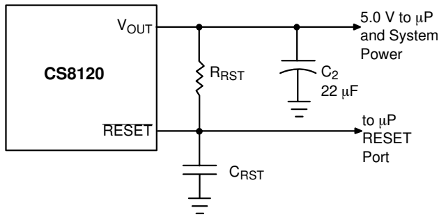
Figure 12. RC Network for RESET Delay Circuitry
