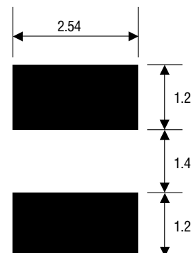
RECOMMENDED PAD LAYOUT PATTERN
