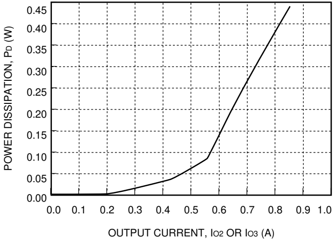
Figure 27. CW025ACL-M Losses Associated with ±15 V Output, Ps2/Ps3
