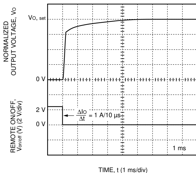
Figure 10. CW025 Dual Output-Series Typical Output Voltage Rise Time with Remote On/Off at V_i = V_{i, \text{nom}} , I_o = 0.8 (I_{o, \max}) and T_c = 25^\circ\text{C}
