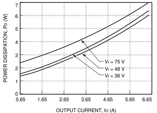
Figure 27. CW030D Power Dissipation vs. Output Current
