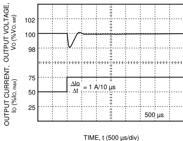
Figure 16. Typical A, B, C, D, F Output Voltage for a Step Load Change from 50% to 75%
