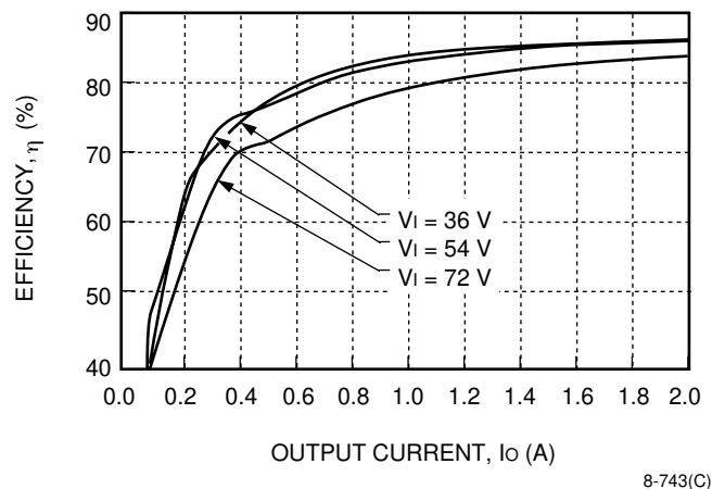
Figure 15. CW030C-M Typical Converter Efficiency vs. Output Current
