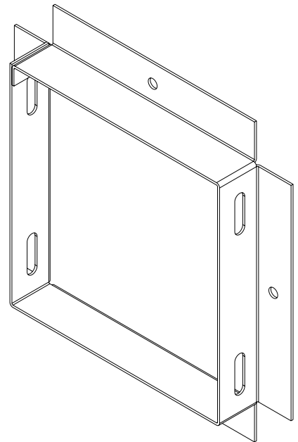
ISOMETRIC VIEW
