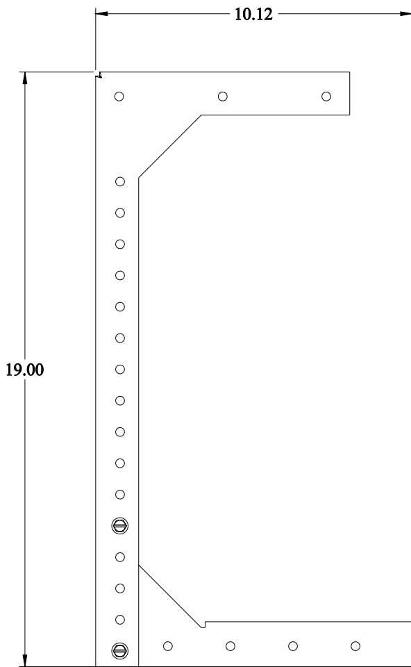
FRONT VIEW
