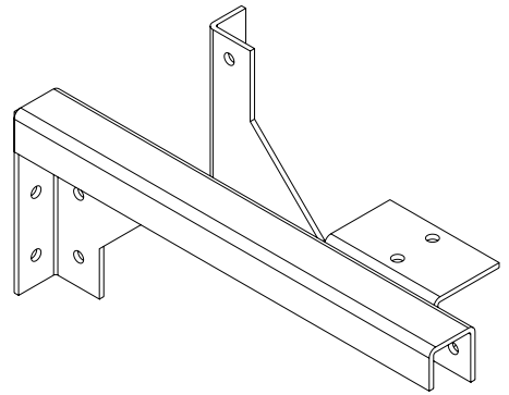
ISOMETRIC VIEW
