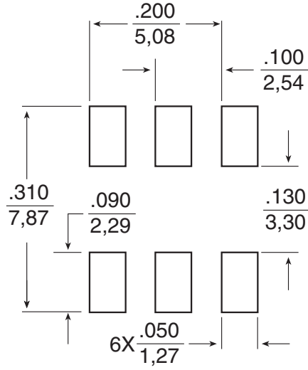
SUGGESTED PAD LAYOUT (Common to all parts)
