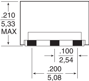
SUGGESTED PAD LAYOUT (Common to all parts)
