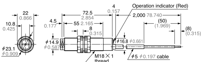
CY-19 Sensor
