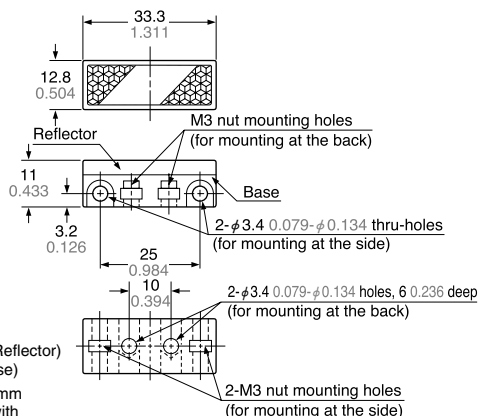
RF-210 Reflector (Optional)
