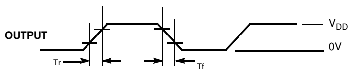
Figure 4. Output Rise/Fall Time (CLKOUT and REFOUT)
