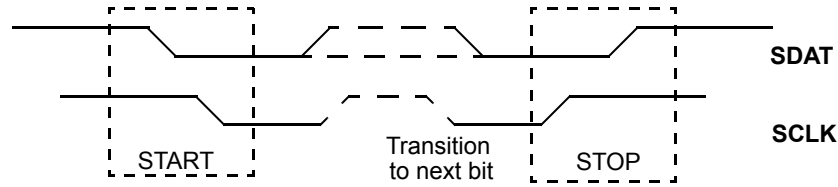
Figure 16. Frame Format (Device Address, R/W, Register Address, Register Data)
