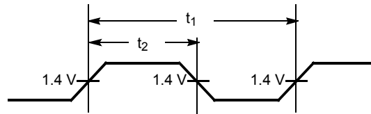
Figure 4. Duty Cycle Timing
