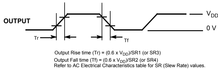
Figure 6. Power Down and Power Up Timing
