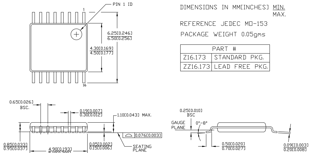
Figure 8. 16-pin TSSOP (4.40 mm Body) Z16.173/ZZ16.173 Package Outline, 51-85091
