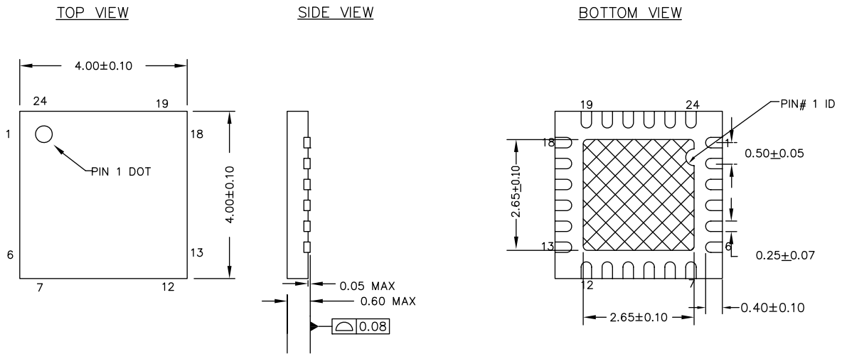
Figure 10. 24-pin QFN ( 4 \times 4 \times 0.55 mm) LQ24A ( 2.65 \times 2.65 E-Pad (Sawn)) Package Outline, 001-13937
