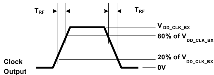
Figure 10. Rise Time = T RF Fall Time = T RF
