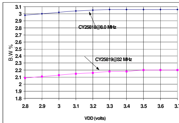
Figure 5. Bandwidth% vs. Vdd
