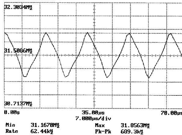
Figure 6. CY25819 Spread Spectrum Profile (Frequency vs. Time) [3]
