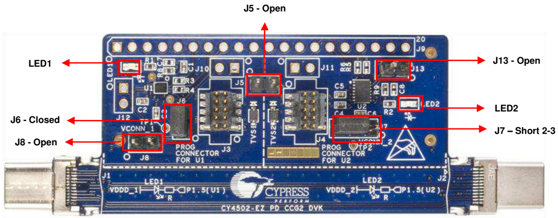
Figure 3-4. CCG2 Single-Chip EMCA Application Jumper Settings
