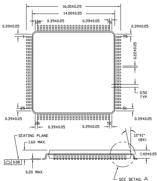
Figure 14. 100-pin TQFP (14 × 14 × 1.4 mm) A100SA Package Outline, 51-85048
