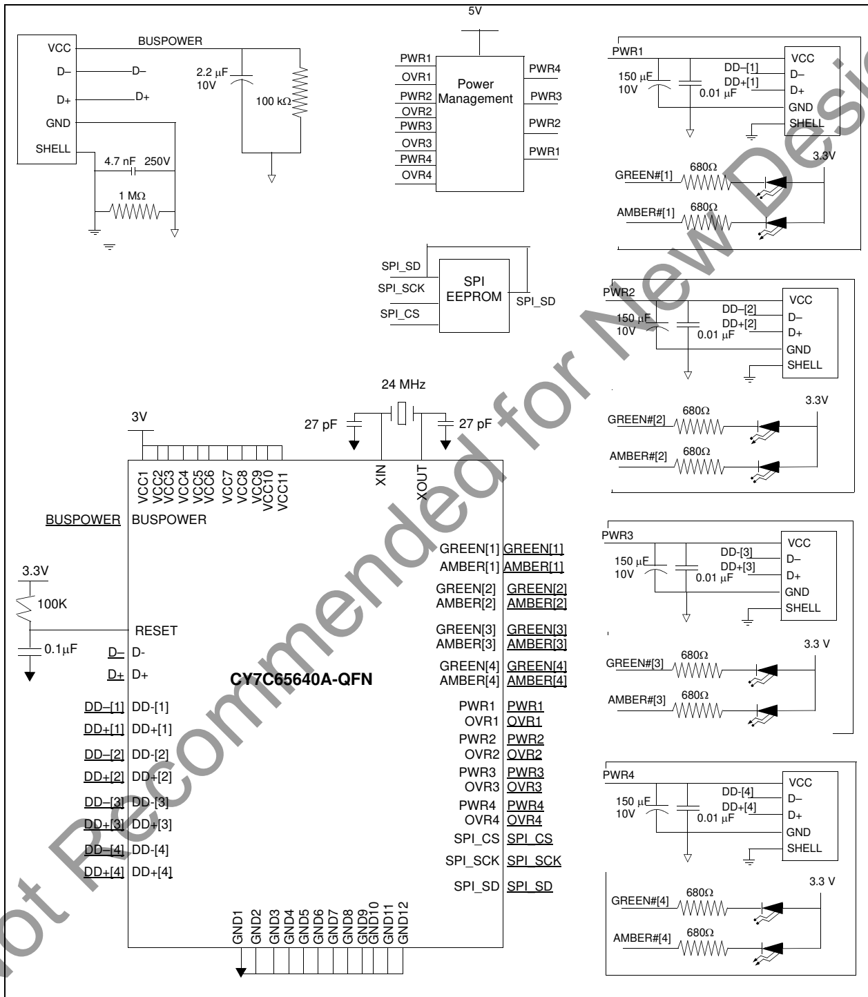
Figure 5. Sample Schematic
