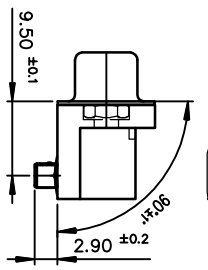
Detail of grounding strip
