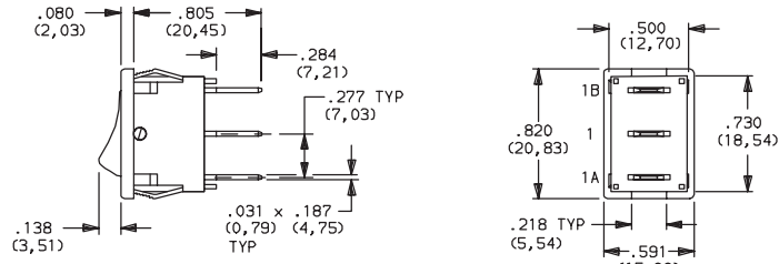
ACTUATOR SHOWN IN POSITION 1
