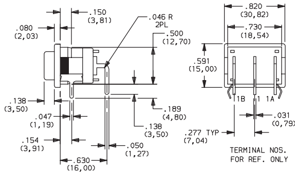
D501J12S2AQA Horizontal Actuation SPDT
