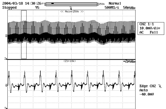
Figure 22 - Ripple, 48 VDC, Full Load. Upper: 50 µs / div, 10 mV / div. Lower: 2 µs / div, 10 mV / div.
