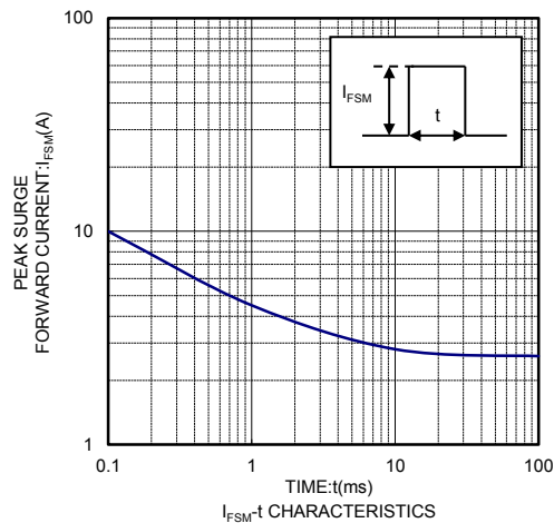
I_{FSM}t CHARACTERISTICS
