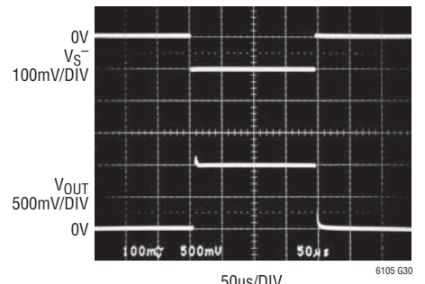
Step Response V_{SENSE} = 0V to 100mV , V_S^+ = 0V
