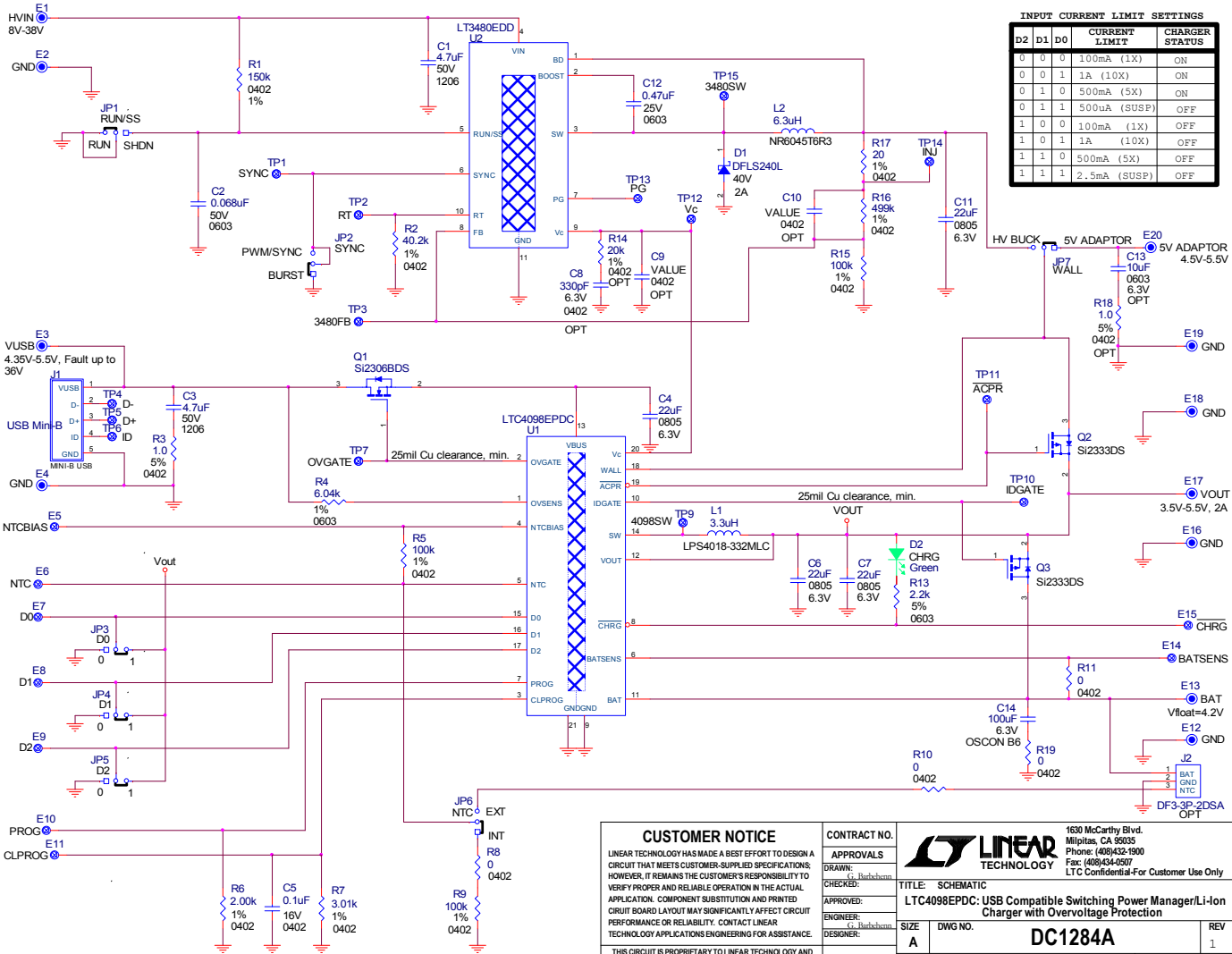
Figure 2: Schematic
