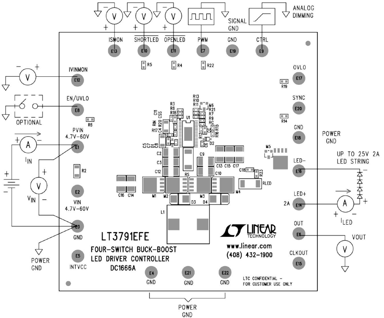
Figure 1. Test Procedure Setup Drawing for DC1666A
