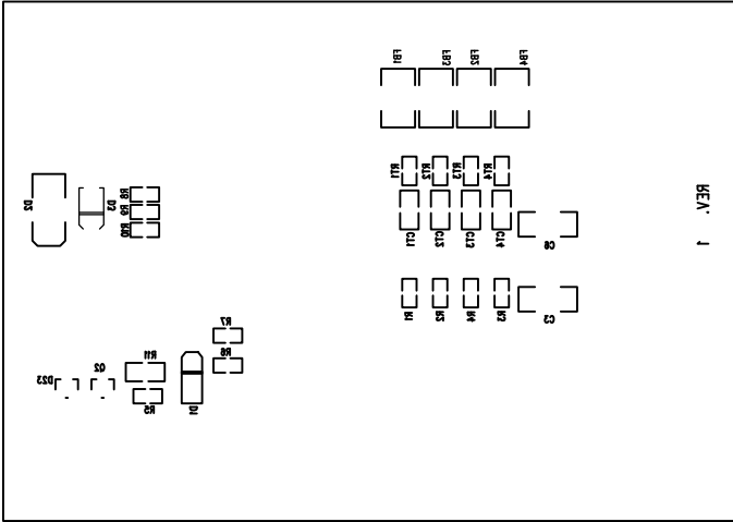
Bottom Silkscreen
