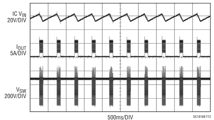
Figure 12. V IN = 277VAC
