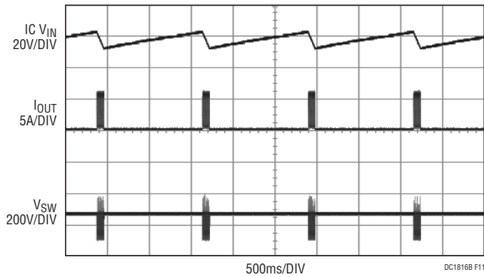
Figure 11. V IN = 120VAC
