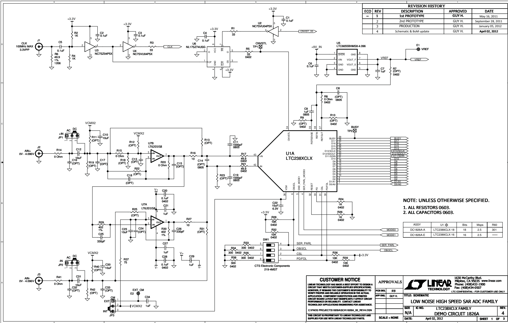
Figure 8. DC1826A Low Noise, High Speed SAR ADC Family
